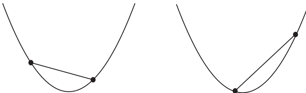
Figure 2. Joining different pairs of points on a curve produces lines with different gradientsV Consider a specific example:
